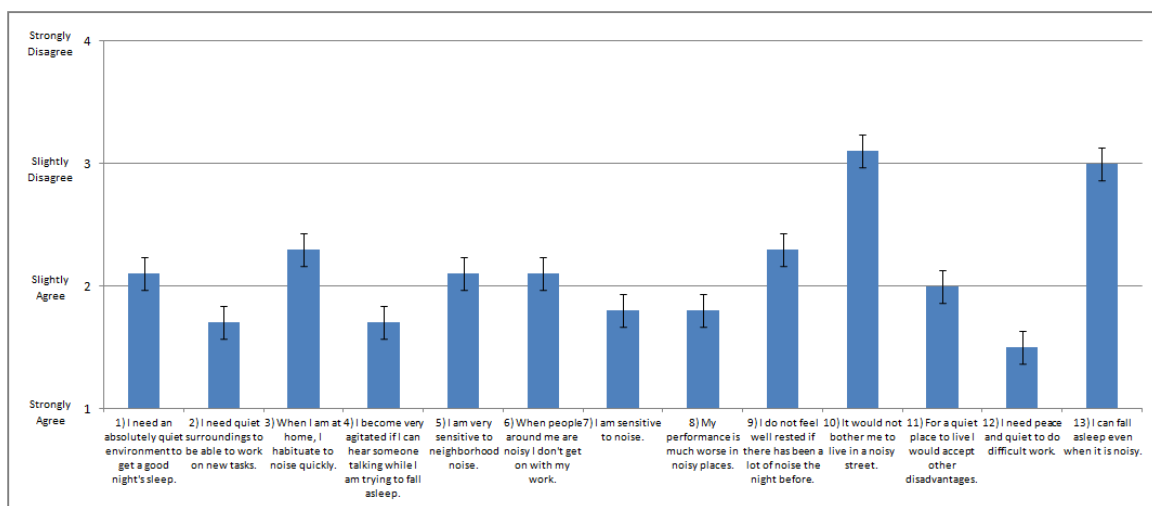
Figure 4.1 Results of the noise sensitivity questionnaires averaged across all subjects. Error bars represent the standard error of the mean.
